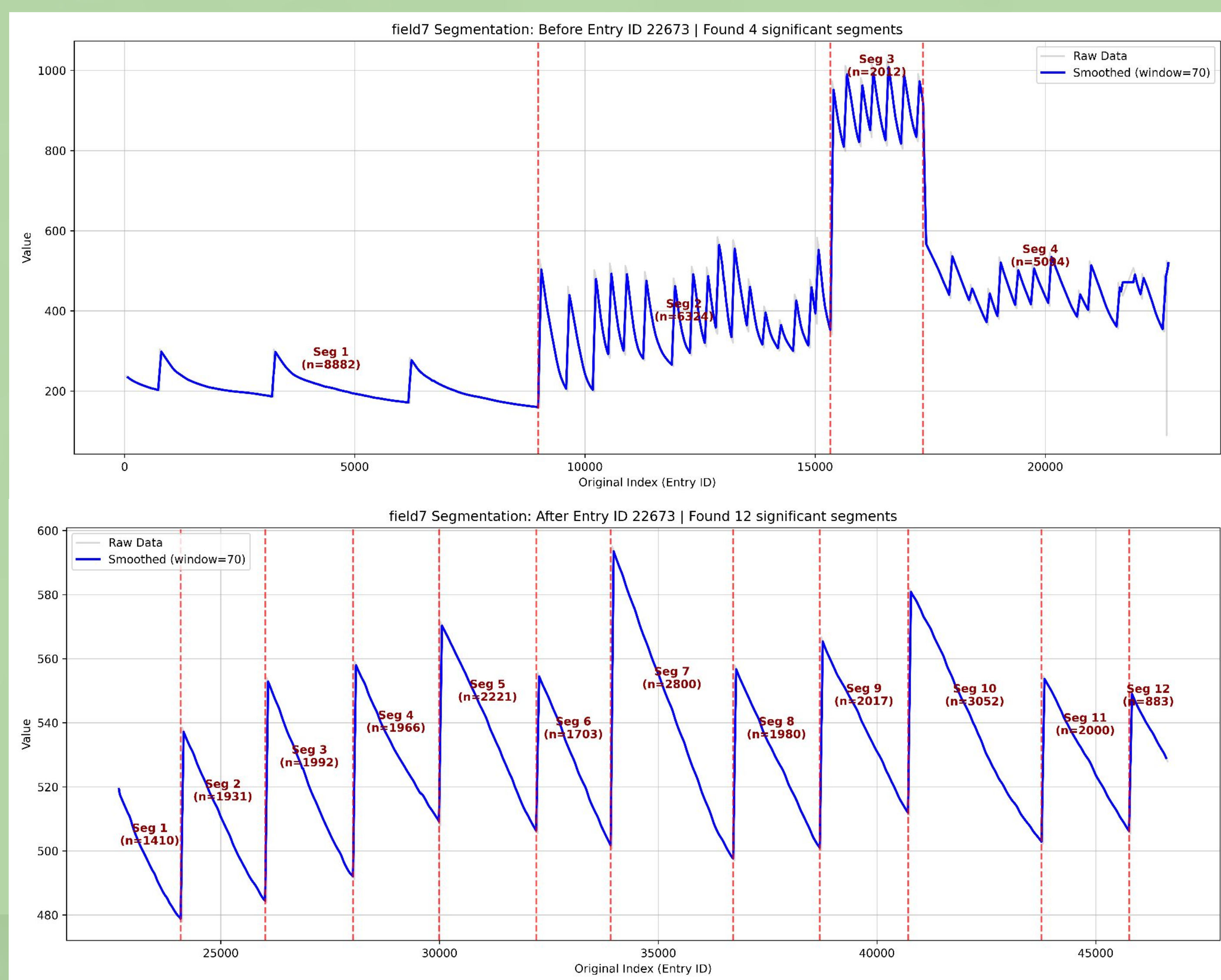
The data series segmented between 30-minute (top) and 5-minute intervals (bottom).
